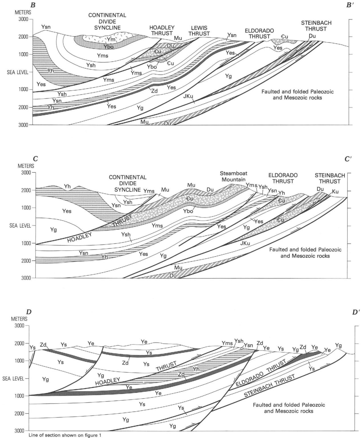
FIGURE 11.—Cross sections of the Hoadley and Eldorado thrust plates, not shown to scale. Approximate position of lines of section are shown in fig. 1; those of section B-B' and C-C' are also shown on fig. 2C. The Belt units in the thrust plates are shown individually on the sections, but are consolidated on the reduced geologic map.
