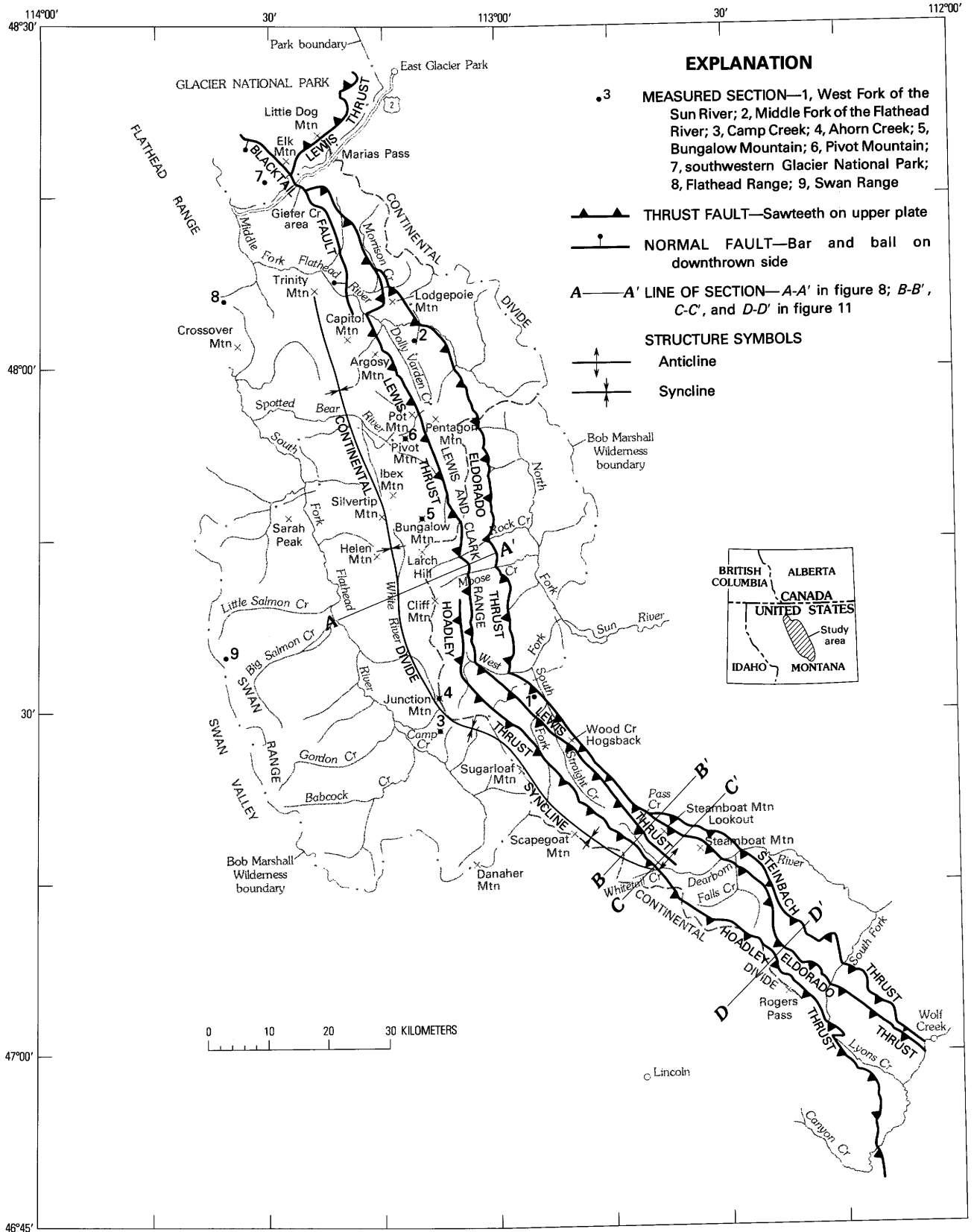
FIGURE 1.—Index map of the area showing the Lewis, Hoadley, and Eldorado thrust faults from Glacier National Park south to Canyon Creek, northwestern Montana.
