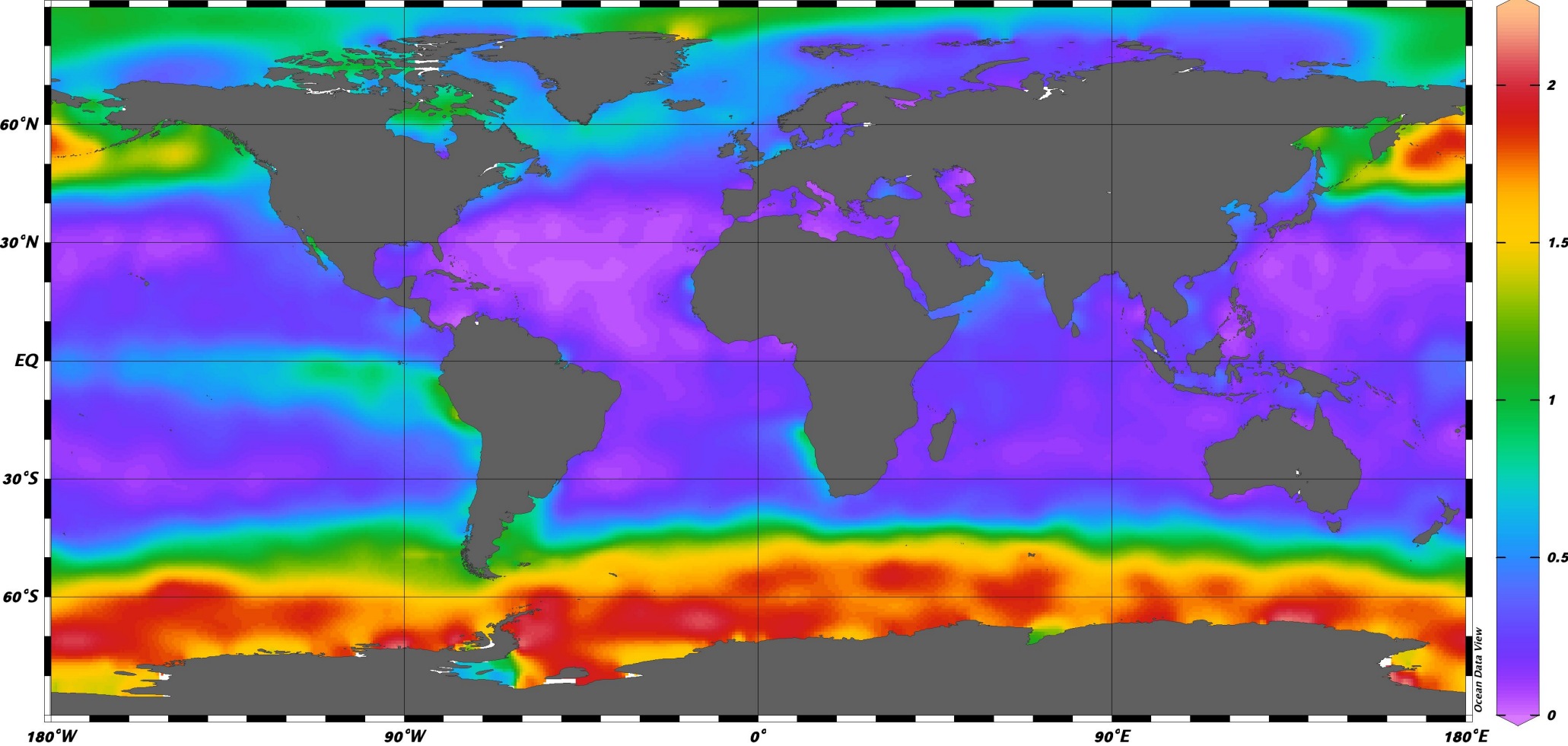
Phosphate [ \mu\text{mol/l} ] @ Depth [m]=0
