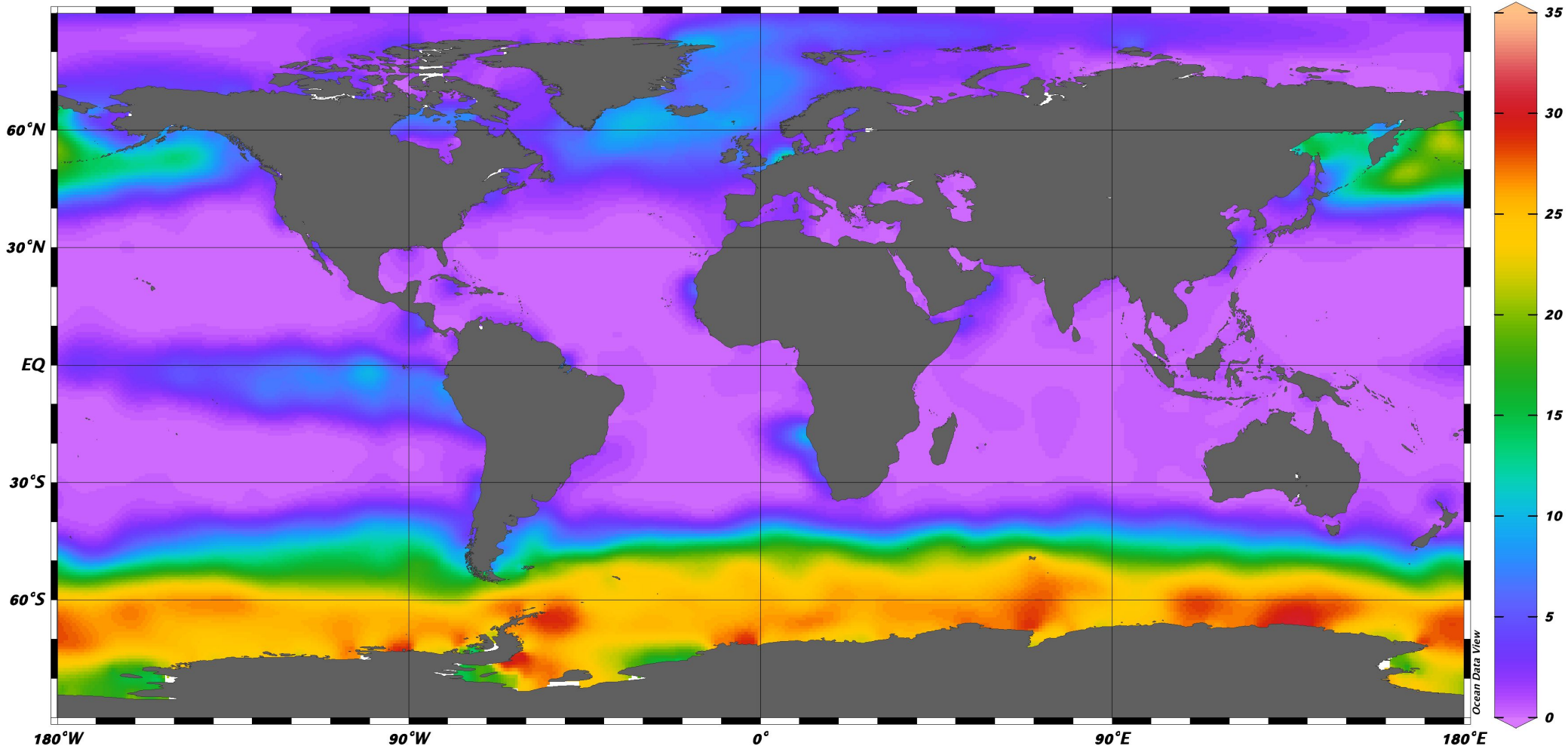
Nitrate [ \mu\text{mol/l} ] @ Depth [m]=0
