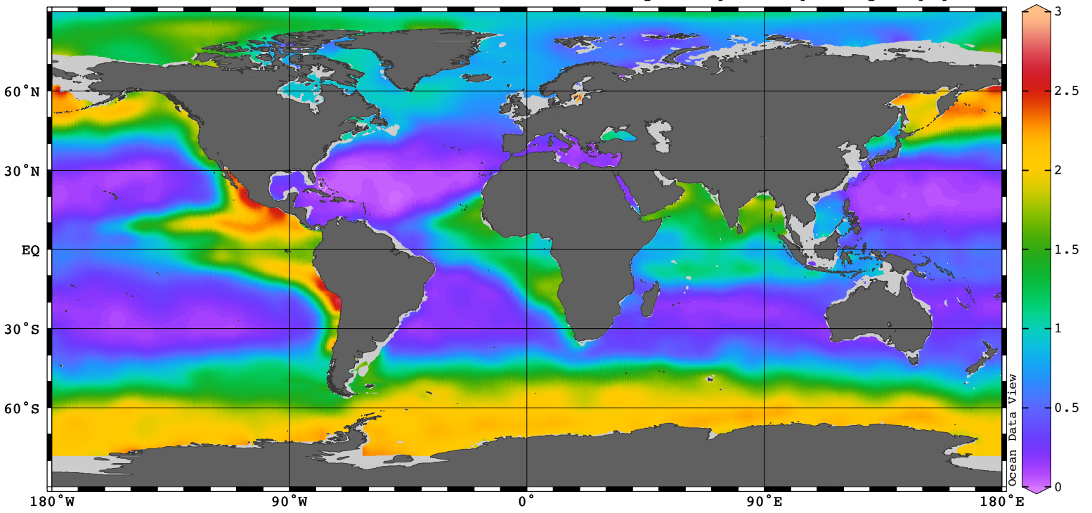
Phosphate [ \mu\text{mol/l} ] @ Depth [m]=100
