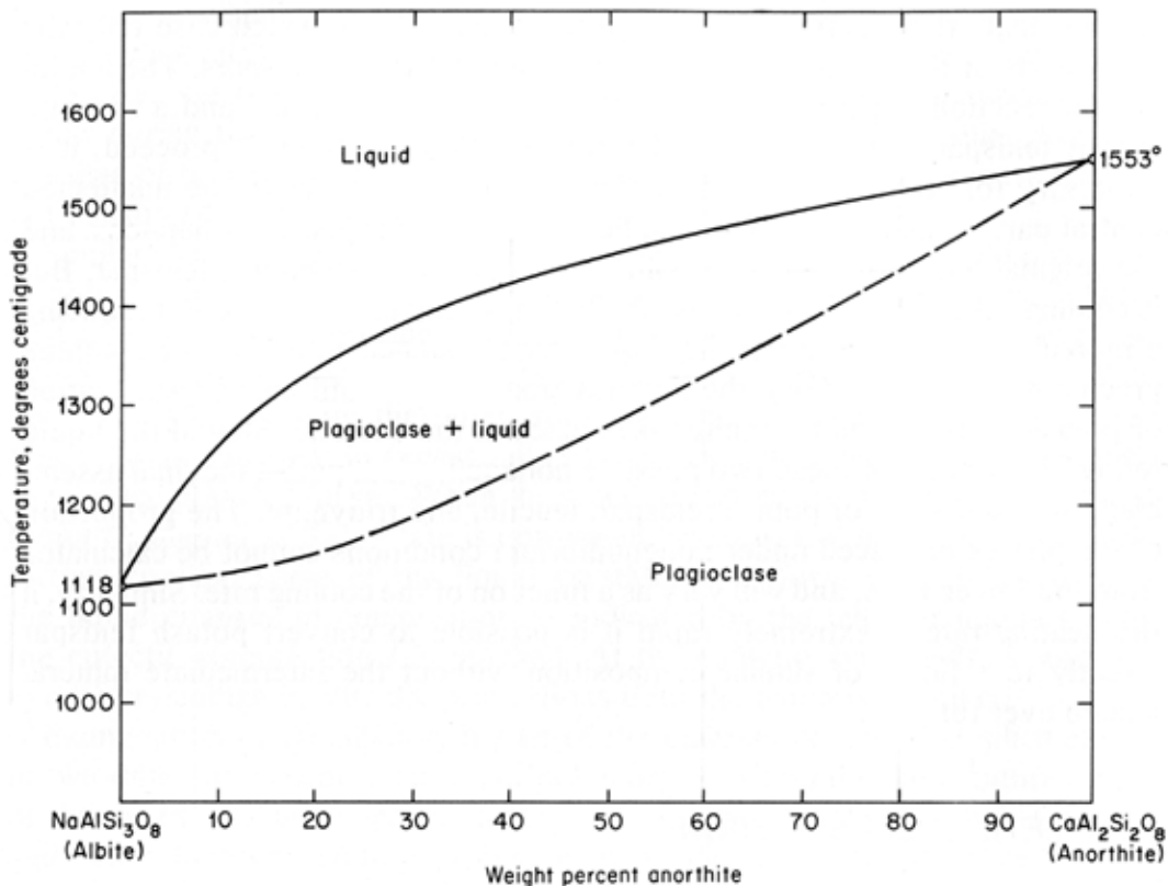
Figure 2. The binary system albite-anorthite at 1 atmosphere pressure after Bowen, 1913.
