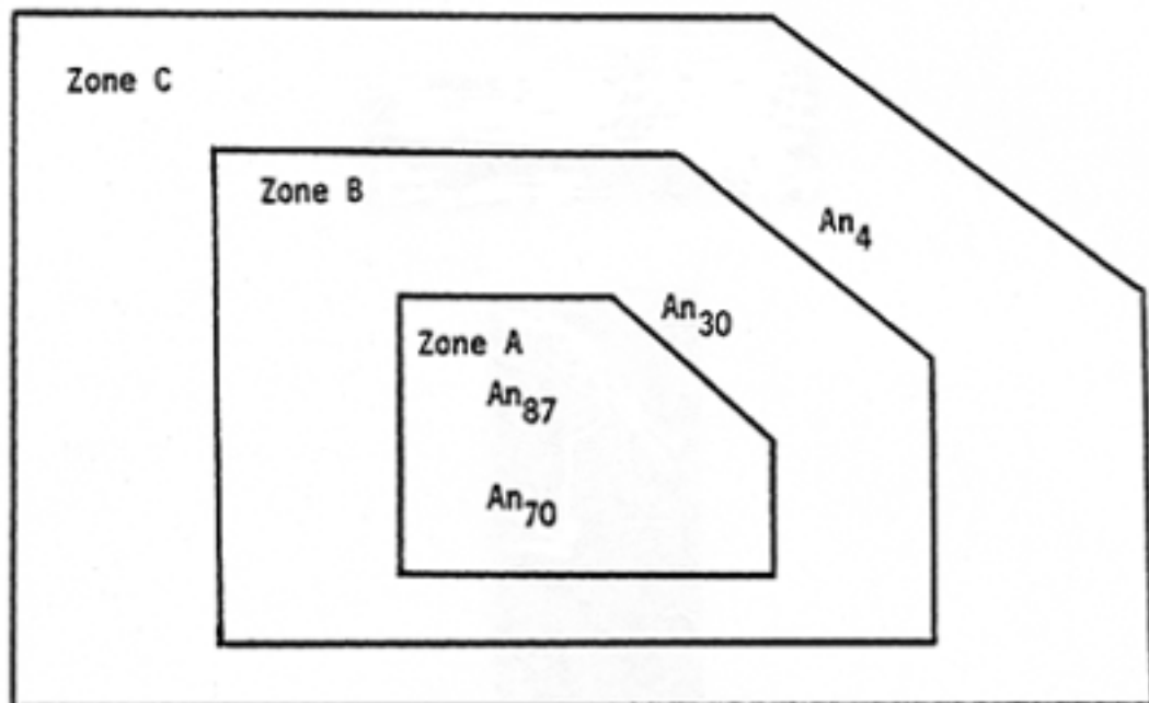
Figure 1. Zoned plagioclase crystal.
