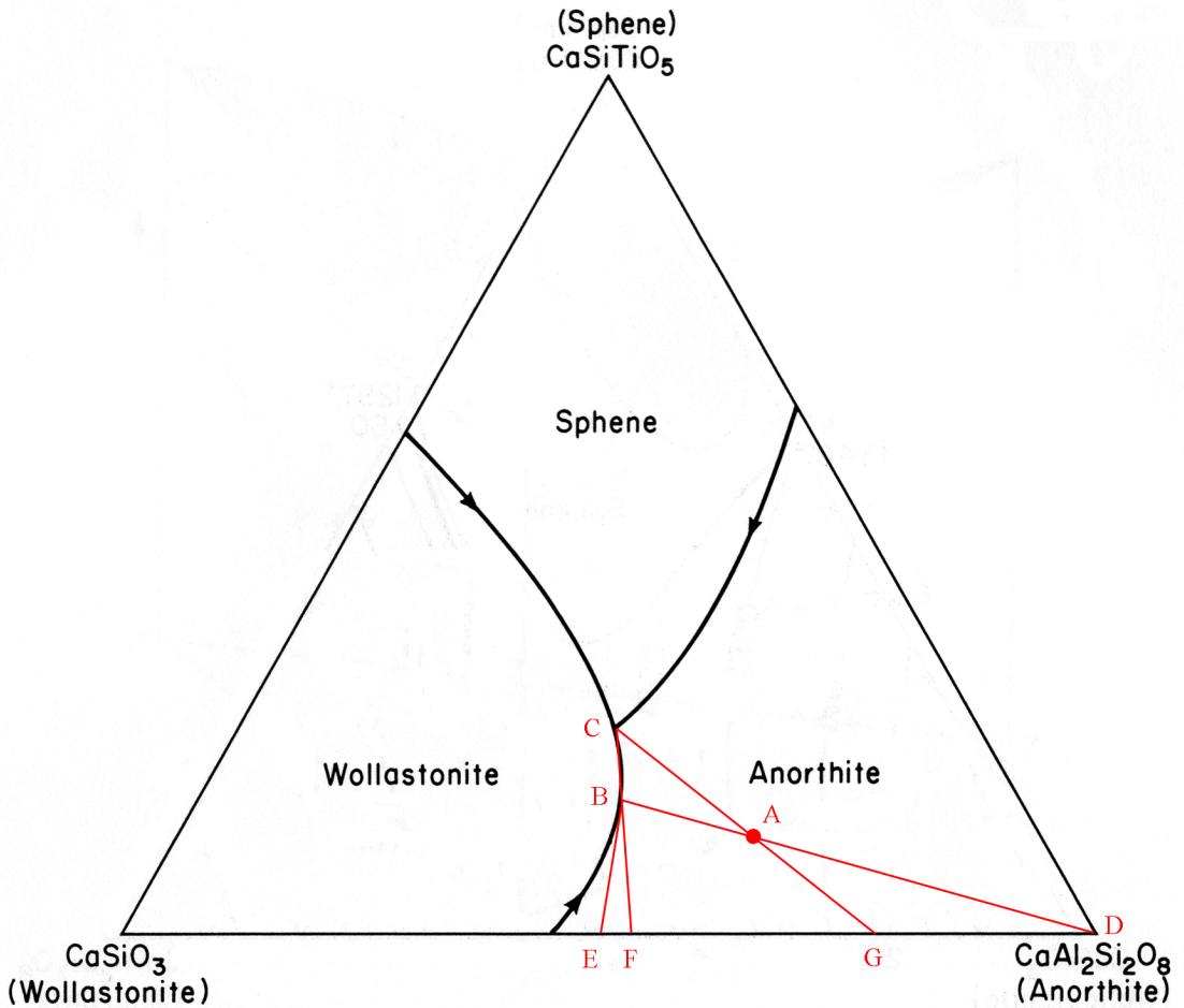
Figure 3. The ternary system wollastonite-anorthite-sphene (after Nishioka, 1935).
